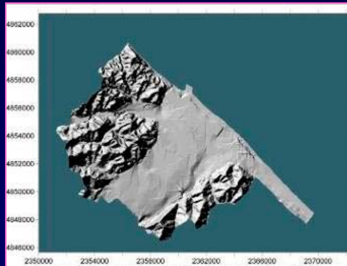
SHADED RELIEF. Light position angle: azimuth 135^\circ , zenit 45^\circ
