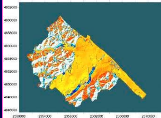
TERRAIN ASPECT MAP
