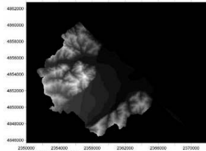
TERRAIN IMAGE MAP
