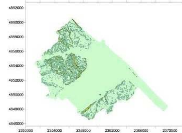
TERRAIN SLOP MAP
